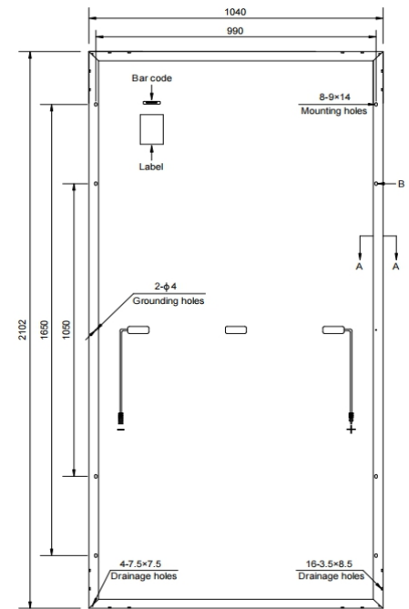
Rear View
